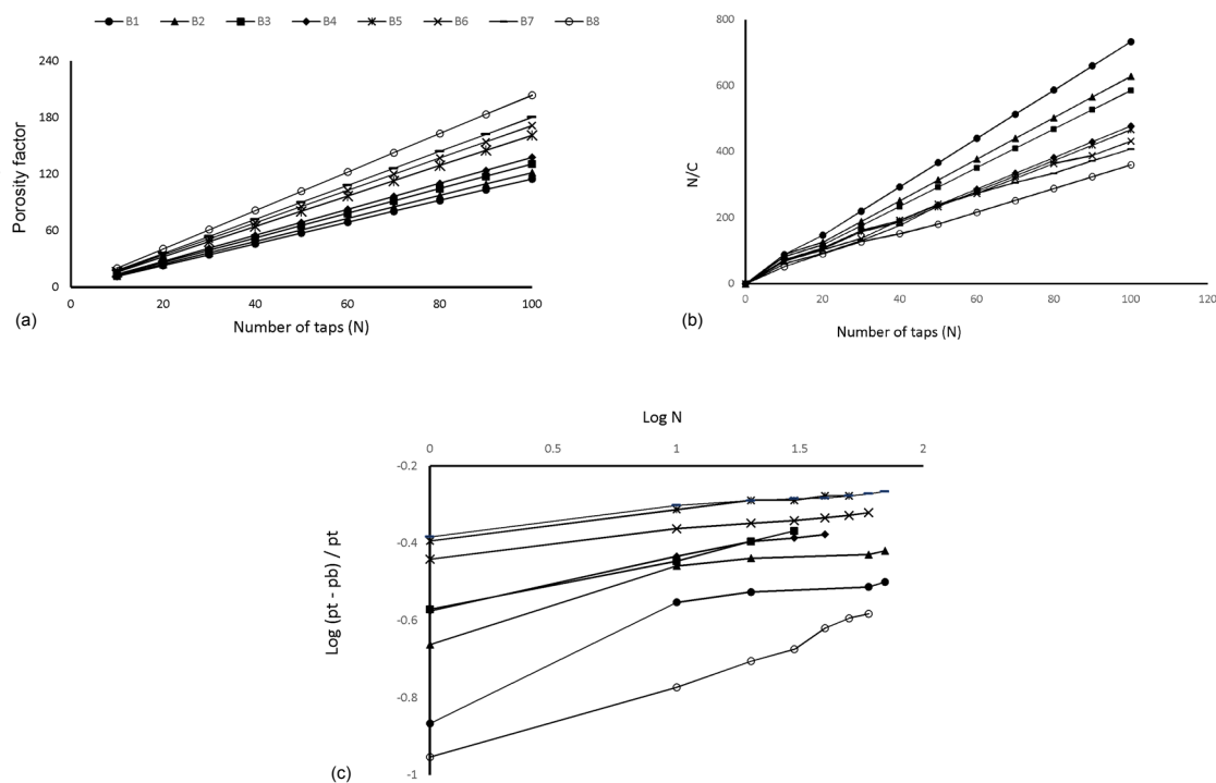
Figure 3 (a) Plots of porosity factors as a function of the number of taps (N), (b) Kawakita plots and (c) Plot of \text{Log} (\rho_T - \rho_B) / \rho_T versus \text{Log} N for pregelatinized Ofada starch, HPMC and the co-processed excipients
